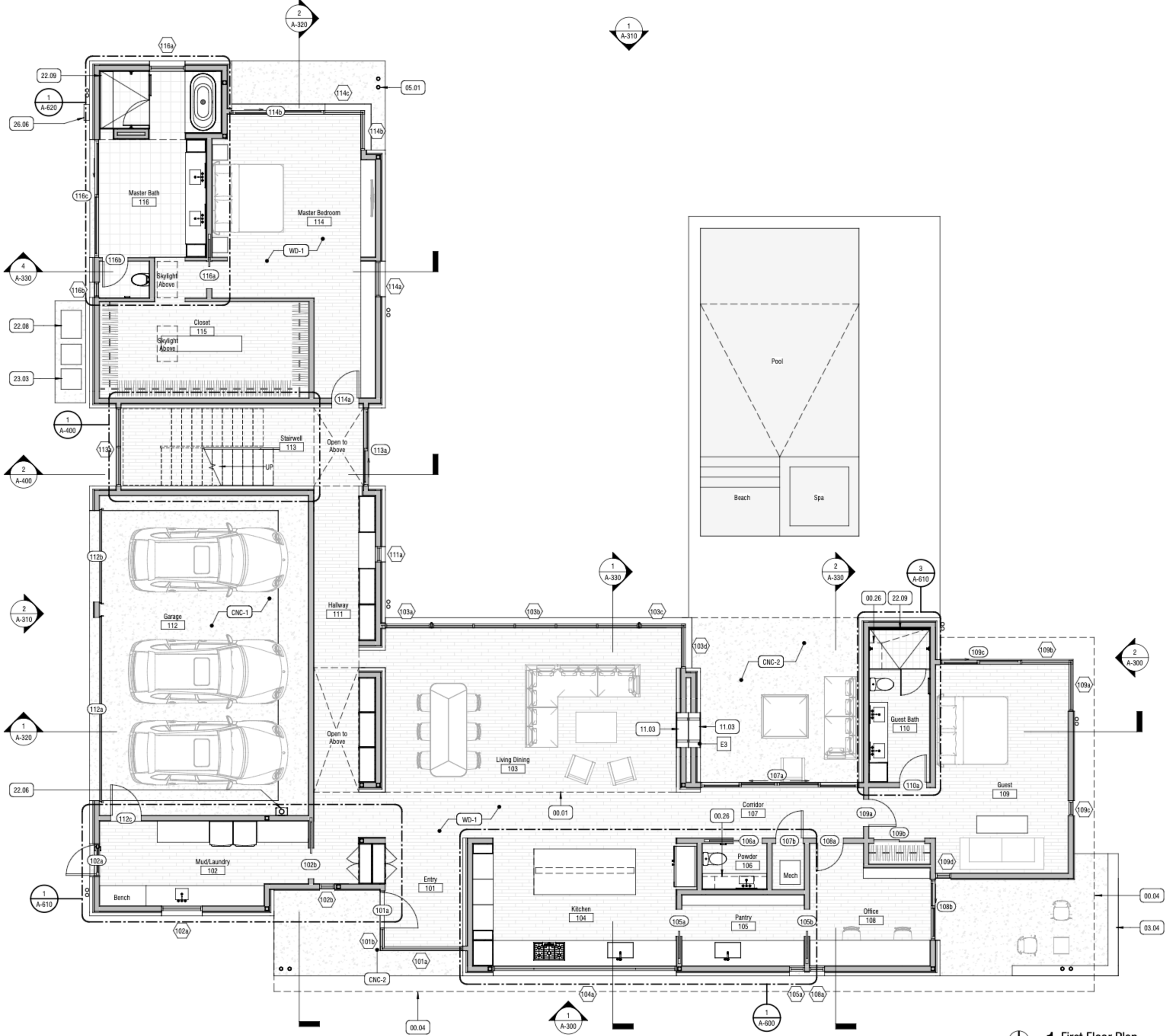
1 First Floor Plan 3/16" = 1'-0"
